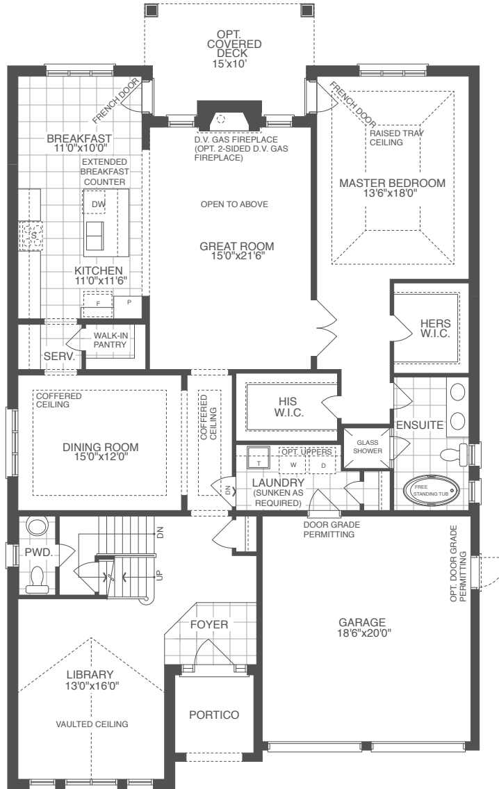
MAIN FLOOR PLAN, EL. 'A'
