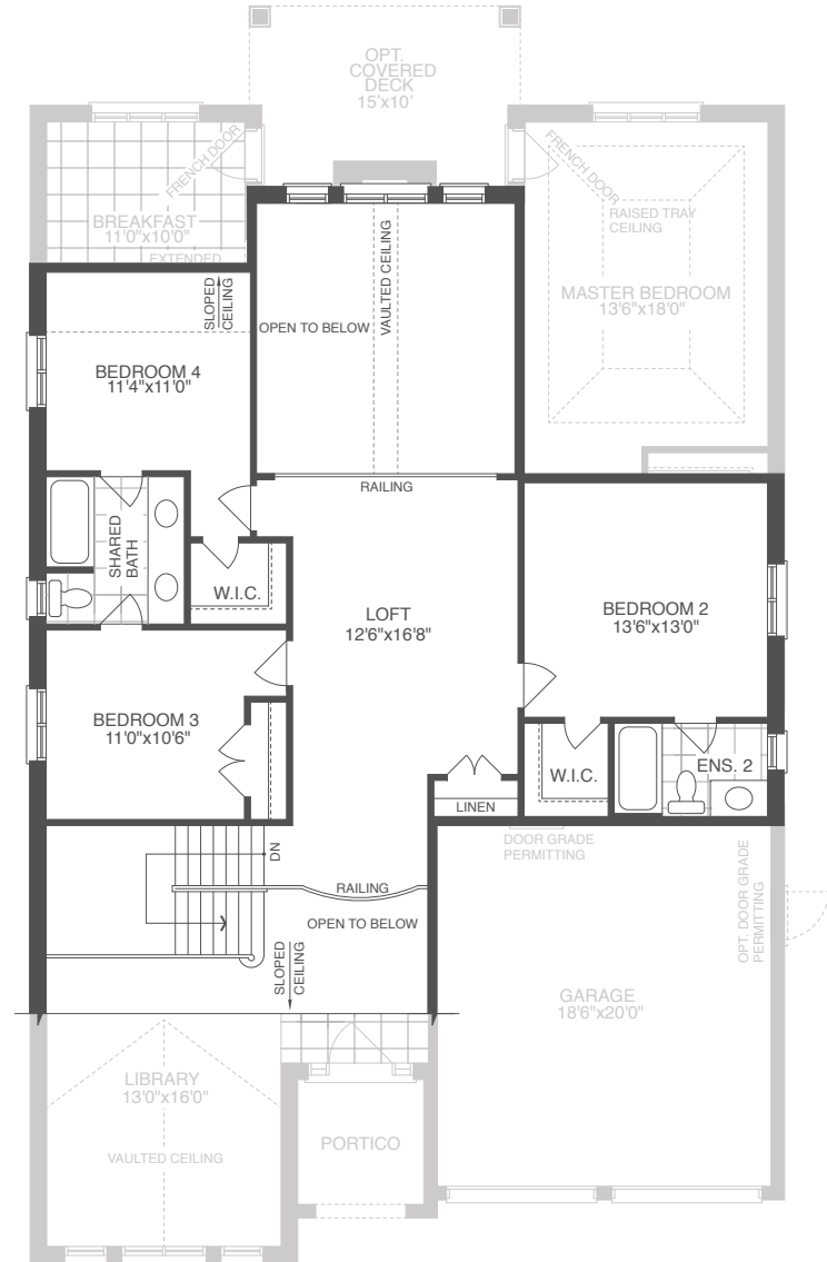
LOFT PLAN, EL. 'A'
